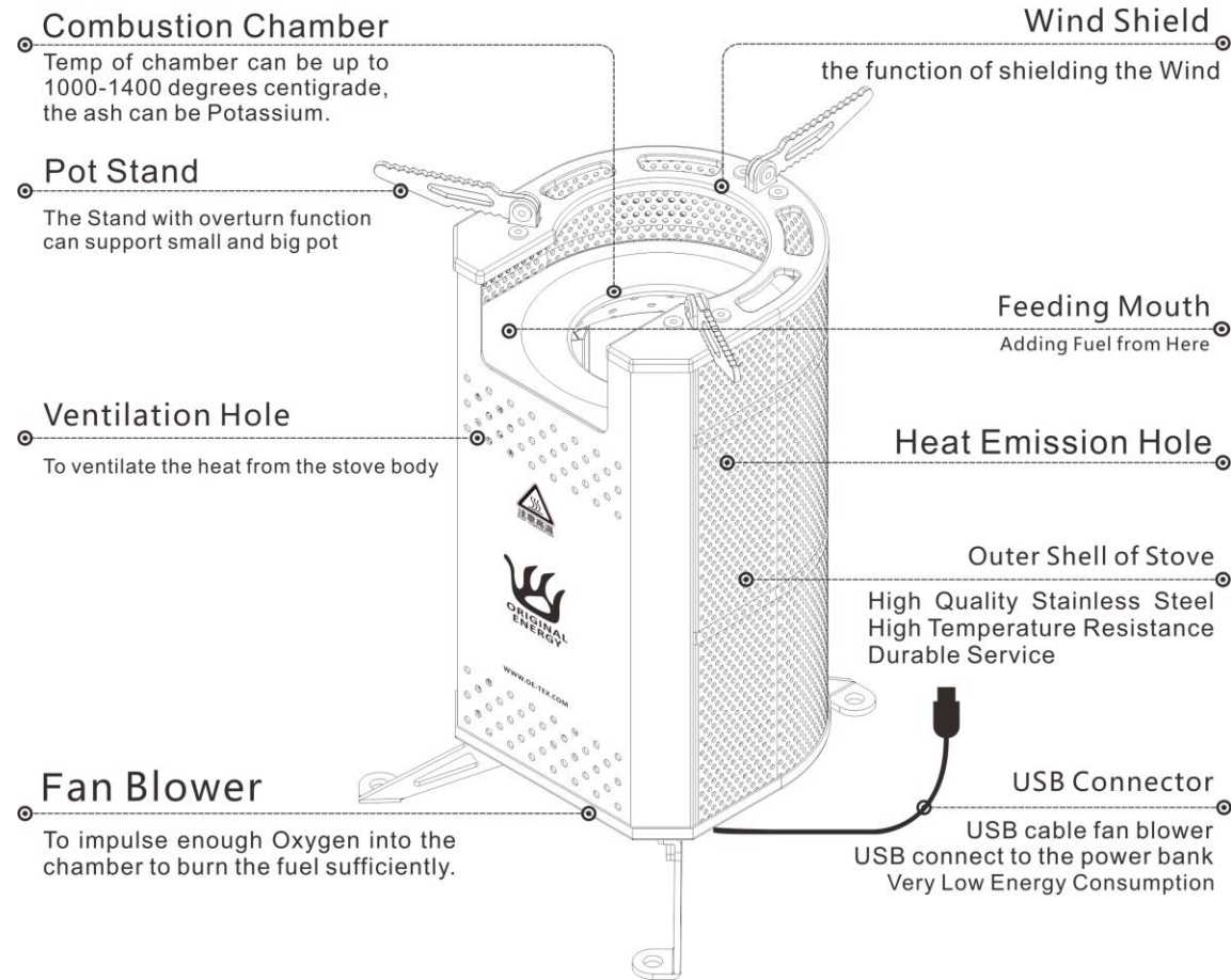
Portable biomass camp stove
